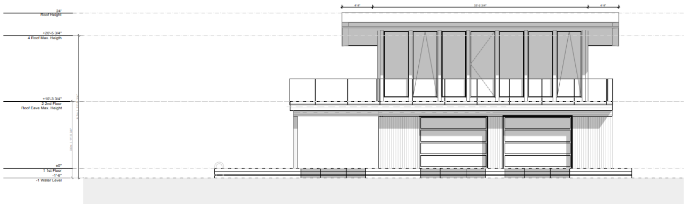
Figure 3: Proposed Waterfront Elevation
