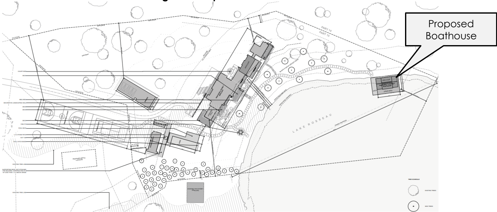
Figure 2: Proposed Site Plan
